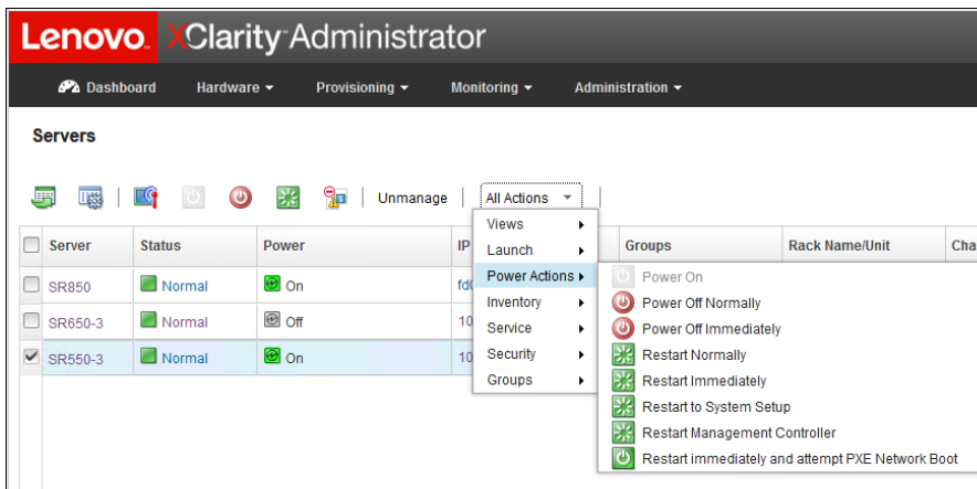
Figure 5. Hardware Management
