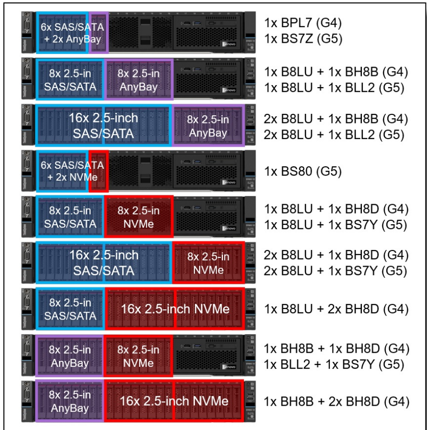
Figure 8. SR665 V3 front drive bay configurations - 2.5-inch drive bays, combinations
