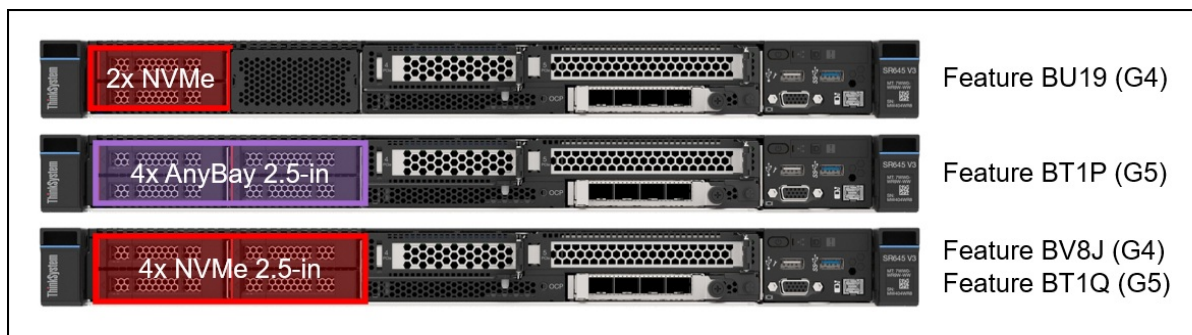
Figure 10. SR645 V3 front drive bay configurations - 2.5-inch drive bays with front PCIe slot support
