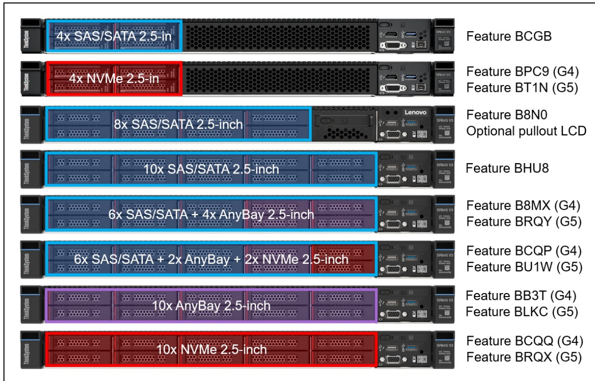
Figure 9. SR645 V3 front drive bay configurations - 2.5-inch drive bays without front PCIe slot support
