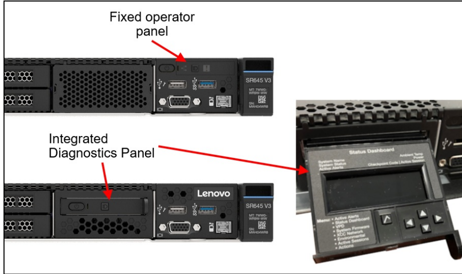
Figure 19. Operator panel choices for the EDSFF and 8x 2.5-inch drive bay configurations
