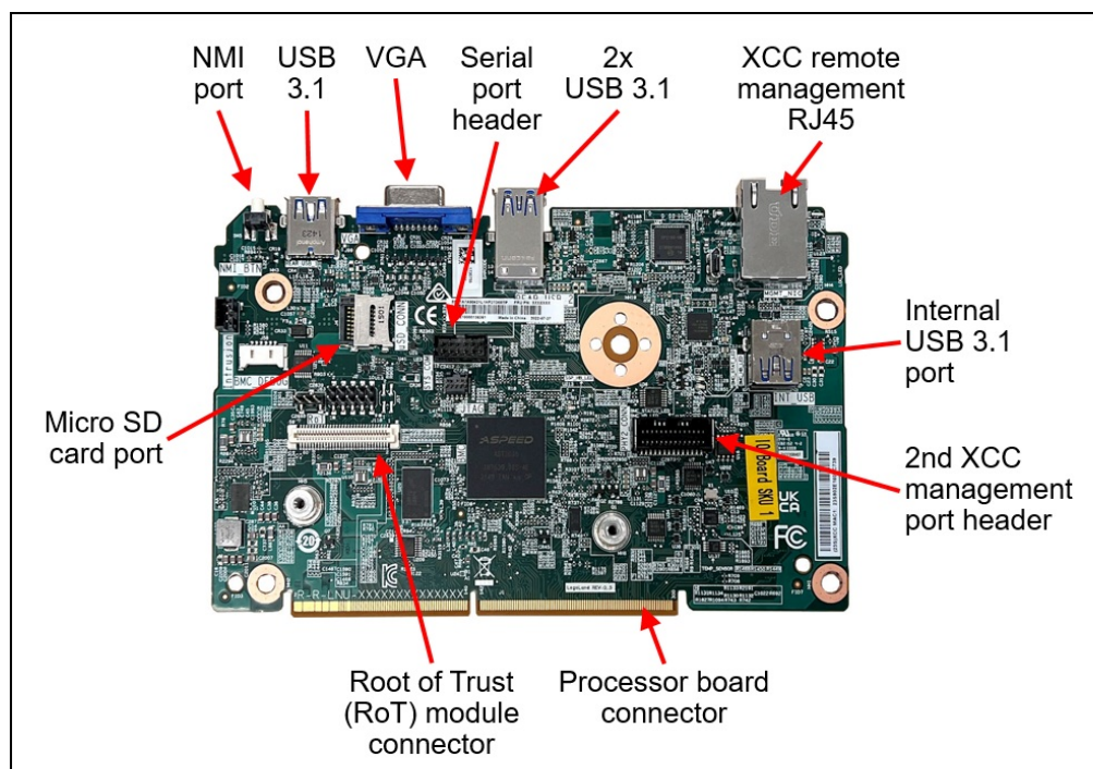
Figure 17. System I/O Board
