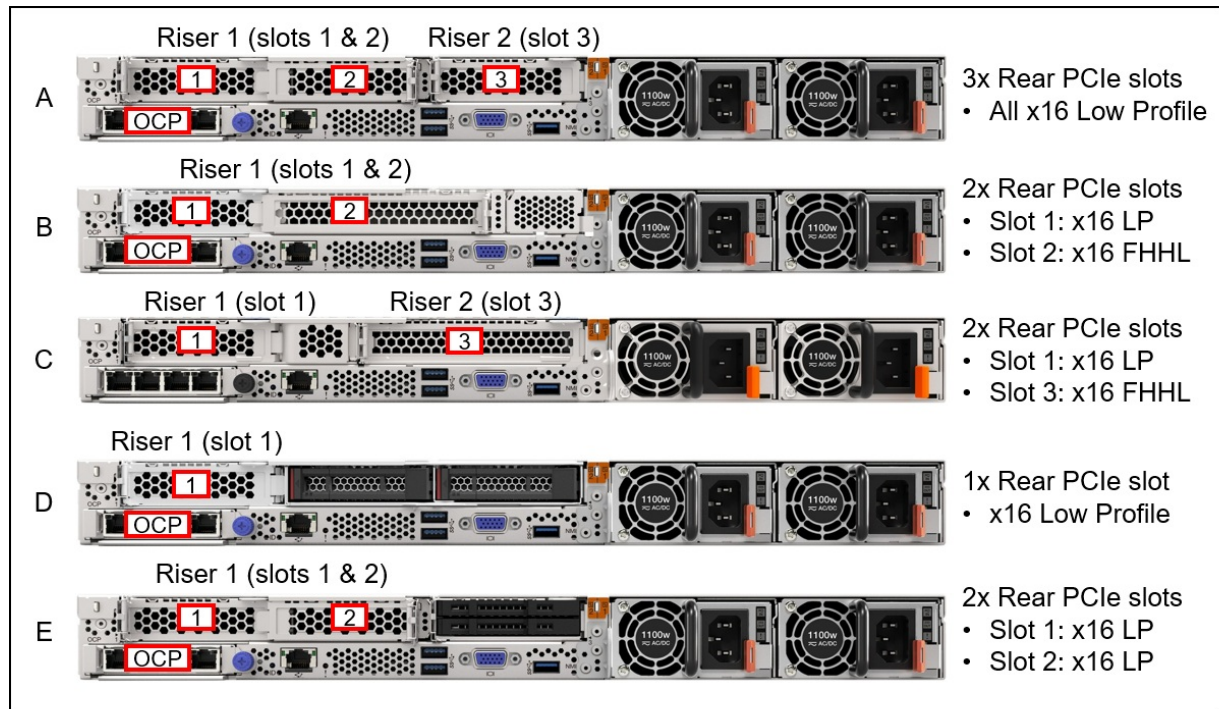
Figure 13. SR645 V3 rear slot configurations
