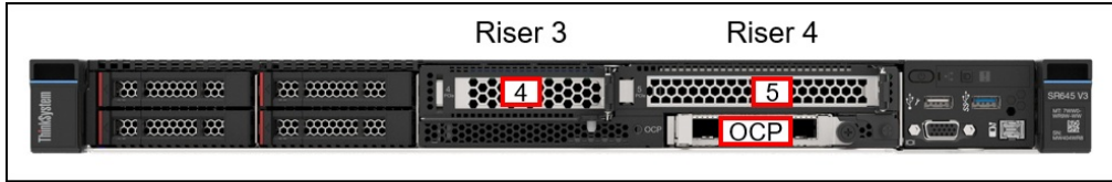
Figure 14. SR645 V3 front slots
