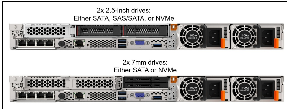
Figure 11. Rear drive bay configurations
