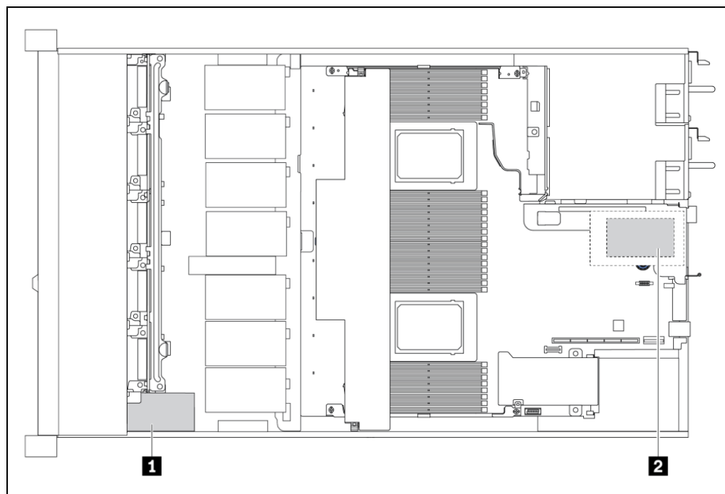
Figure 12. Location of the supercaps in the SR645 V3
